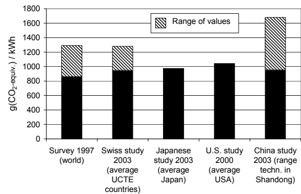
Fig. 1: GHG emissions from coal-power plants and associated fuel cycles according to different studies.
