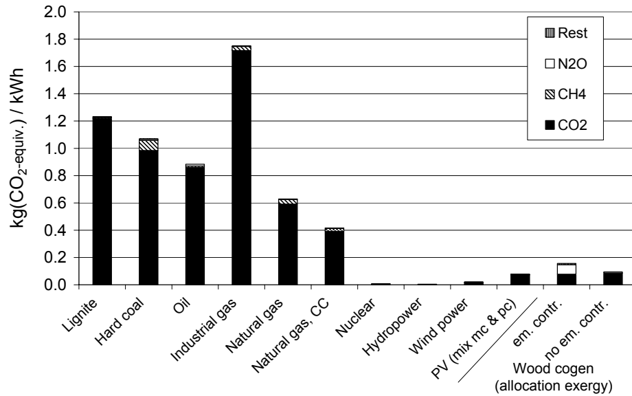
Fig. 6: Overview of full chain GHG emissions for different electricity generation systems [1]. Lignite, hard coal, oil, industrial gas, natural gas, and nuclear refer to energy systems associated with average UCTE power plants for the year 2000. Natural gas CC refers to combined-cycle power plants utilising the current best technology, and with gas supplied by the European high-pressure grid. The renewables — hydropower, wind power, photovoltaic, wood — refer to data pertinent to Switzerland.
