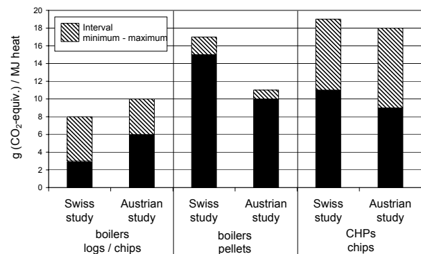
Fig. 5: GHG emissions for wood heating systems in Central Europe.
