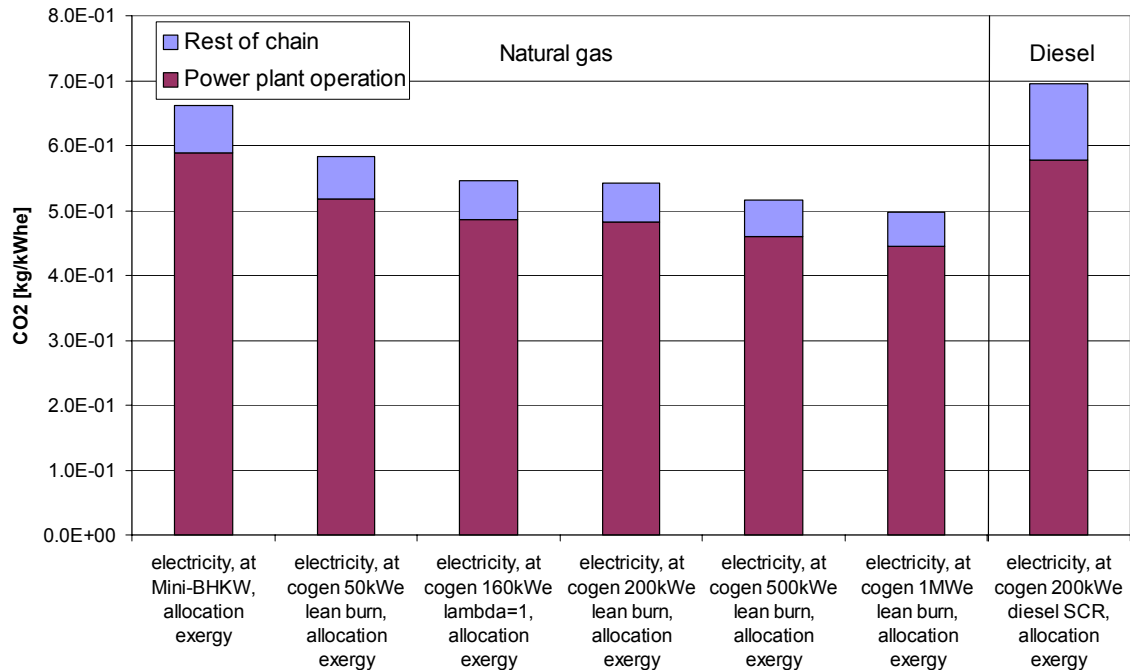
Fig. 4: CO 2 emissions per kWh e from modern small cogeneration plants of different capacity and technology. Lambda=1: Cogeneration unit with three-way catalyst. Mini-BHKW: 2kWe small device designed for a small house. SCR = Selective Catalytic Reduction. The allocation to electricity is based on the exergy of electricity and heat, assuming an upper temperature of about 80°C for heat [1].
