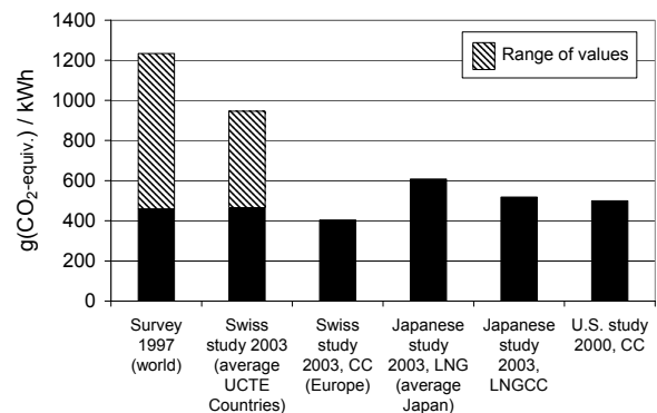
Fig. 2: GHG emissions from gas power plants.
