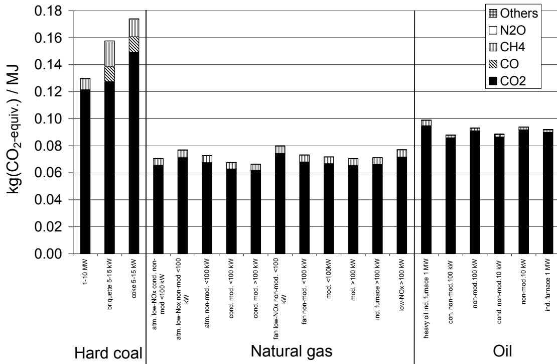
Fig. 3: GHG emissions from fossil-fuel heating systems operating in the year 2000 in Central Europe. Atm. = Atmospheric boiler; Fan = Fan burner; Mod. = Modulating boiler; Cond. = Condensing boiler; Ind. furnace = Industrial furnace; Low-NOx refers to boilers built in the early 1990s; Modulating boilers refer to the most modern technology on the market [1].
