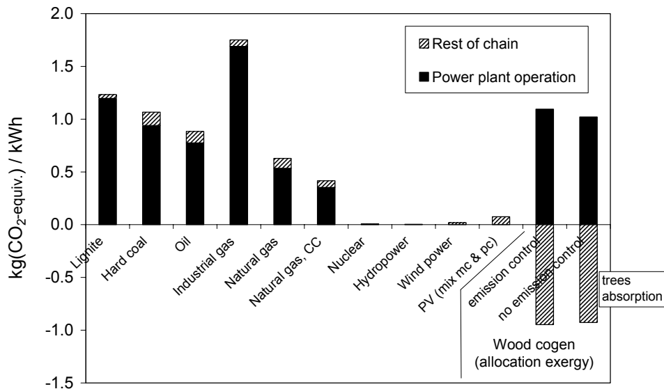
Fig. 6: Overview of full chain GHG emissions for different electricity generation systems [1]. Lignite, hard coal, oil, industrial gas, natural gas, and nuclear refer to energy systems associated with average UCTE power plants for the year 2000. Natural gas CC refers to combined-cycle power plants utilising the current best technology, and with gas supplied by the European high-pressure grid. The renewables — hydropower, wind power, photovoltaic, wood — refer to data pertinent to Switzerland.
